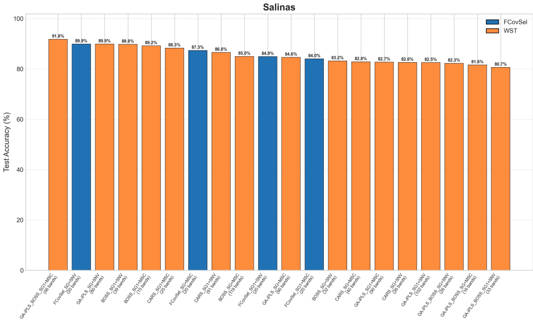
All Methods - 3D-CNN Test Accuracy (Sorted) Block-Based Spatial Split + Data Augmentation
